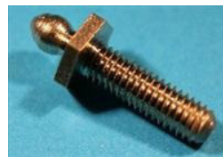
TENAX18-5/8.UNFP QTY:4 Tenax fastener, length 5/8" with a UNF thread size. General application
