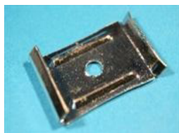
BSF069P QTY:16 Moulding clip for 22.8mm moulding gap. Humber, Hillman Hunter range.
