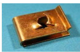
SNU3489P QTY:30 No10 'U' nut, length 19.6mm, width 12.7mm, panel range 3.17mm-3.42mm. General application.
