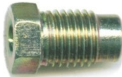
BN15P QTY:25 Brake Nuts 10mm x 1.25mm pitch long male, for 3/16" pipe
