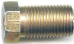
BN21P QTY:25 Brake Nuts 10mm x 1mm pitch full threaded long male , for 3/16" pipe
