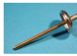
BSF078P QTY:15 Round 'Tuckers' moulding clip for 11.3mm moulding gap and 3.2mm panel hole. MG, and general application
