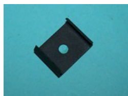
BSF126P QTY:25 Moulding Clip for a 16.7mm moulding gap. Vauxhall range.
