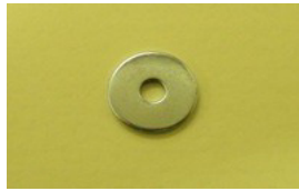
BSF130P QTY:25 Washer 20mm diameter, hole size 5.0mm. Mini petrol tanks and general application.
